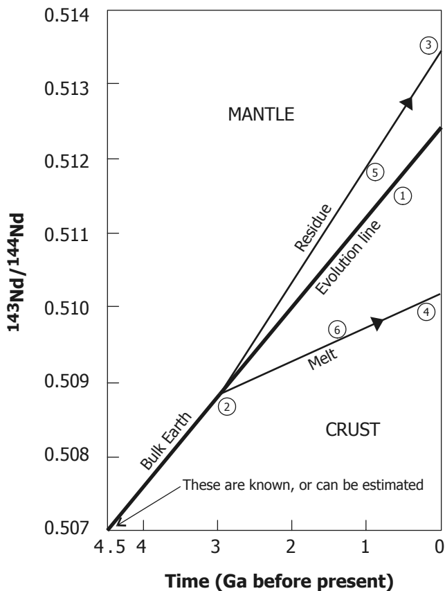
Figure 1. Nd Isotope Evolution of the Earth
